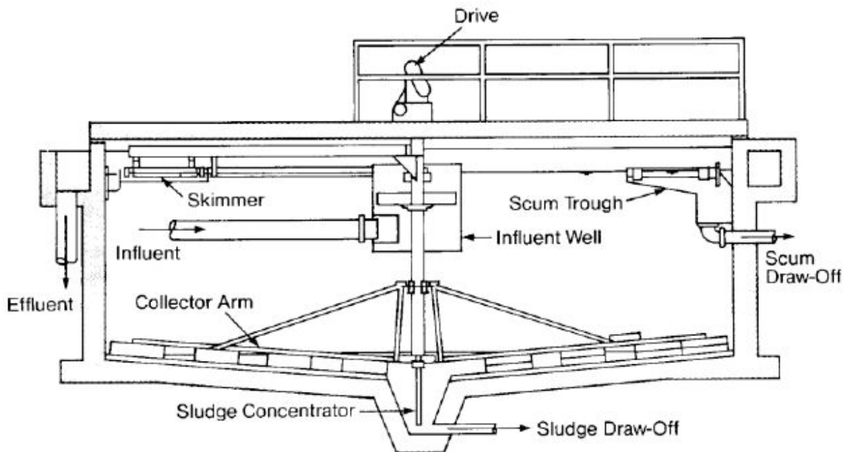
Mechanical clarifier
