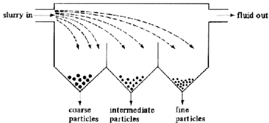
Settling tank
